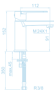
Monomando Lavabo Alto Helena Ref. HL109N
