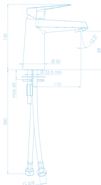
Monomando Lavabo Milano Ref. SY97118/2 CR
