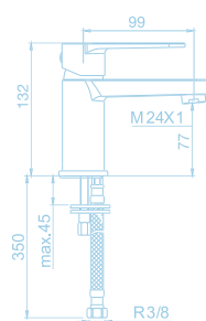
Monomando Lavabo Helena Ref. HL107N
